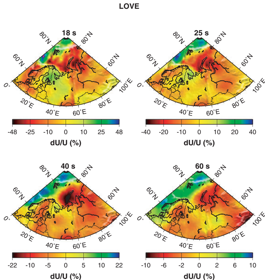
Figure 5. Results of the 2-D inversion for the group velocities of Love waves with period of 18, 25, 40 and 60 s. The maps present the 2-D distribution of the inverted group velocities as deviations from the average velocity across the region (in per cent).
