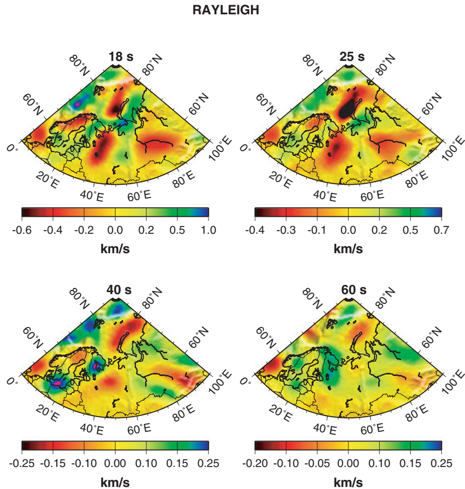
Figure 8. Difference between the initial and newly inverted group-velocity maps of Rayleigh waves with period of 18, 25, 40 and 60 s (in \text{km s}^{-1} ).
