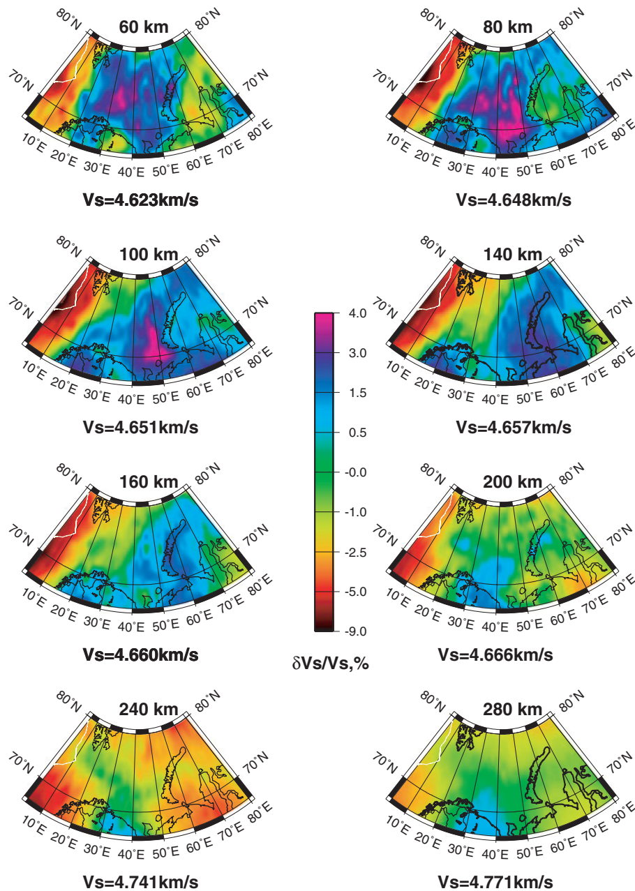
Figure 11. Results of the 3-D tomographic inversion: isotropic shear wave velocities V_s = (V_{sv} + V_{sh})/2 at different depths relative to the 1-D model Barey. The reference S -velocities are presented below each map.
