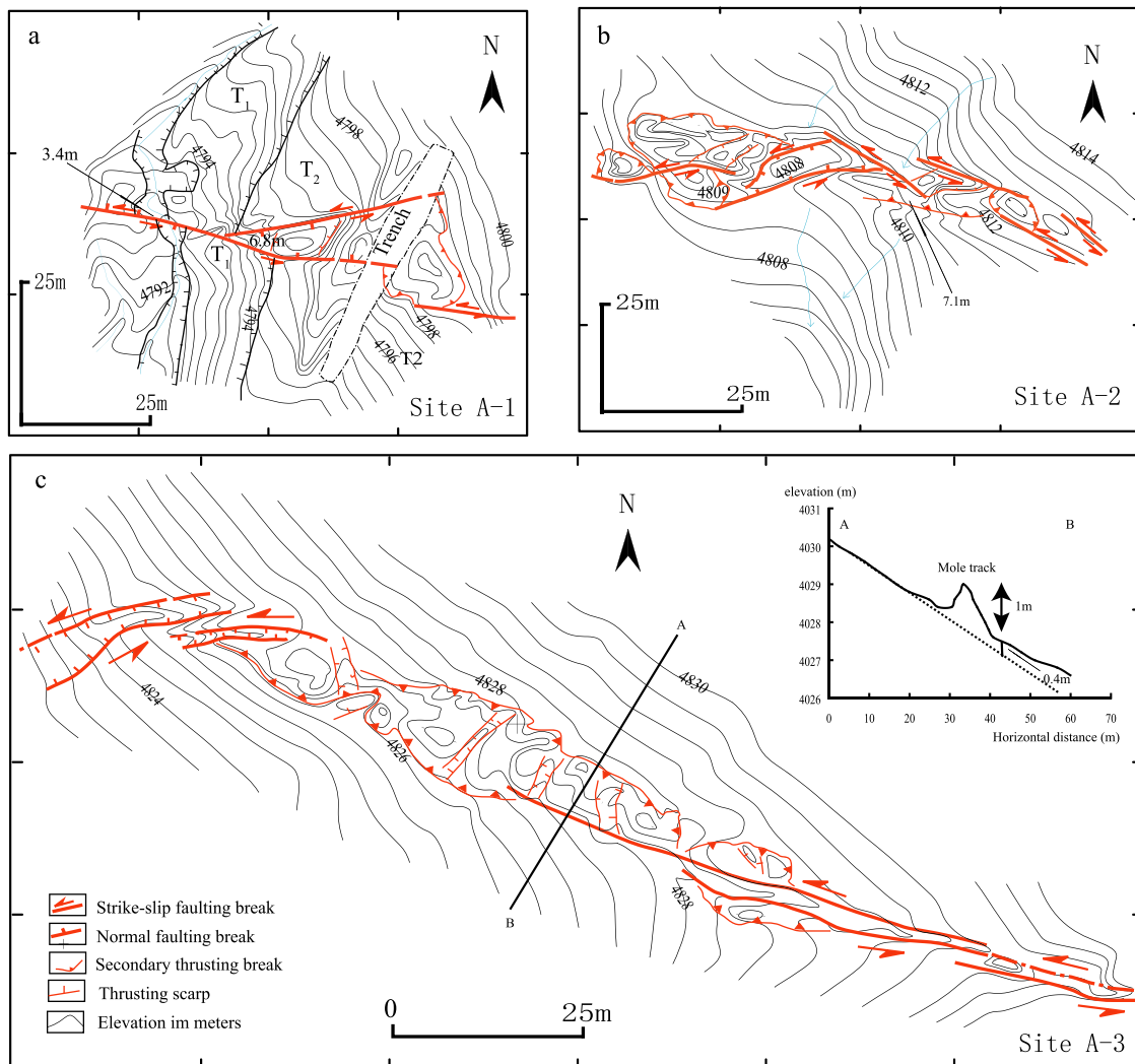
Figure 12. Measured topographic map showing surface rupture pattern and coseismic left-lateral offset features on the Yuzhu Feng subsection. (a) Offset terrace risers at the site A-1 ( 35.668^{\circ}\text{N} , 94.070^{\circ}\text{E} ). (b) En echelon strike-slip breaks, mole tracks and pull-aparts, as well as the offset fan surface and small gullies at site A-2 ( 35.668^{\circ}\text{N} , 94.069^{\circ}\text{E} ). (c) En echelon strike-slip breaks, mole tracks and pull-aparts, as well as the offset fan surface at the site A-3 ( 35.668^{\circ}\text{N} , 94.0727^{\circ}\text{E} ). The inset map shows cross section of a mole track and southern wall up.
