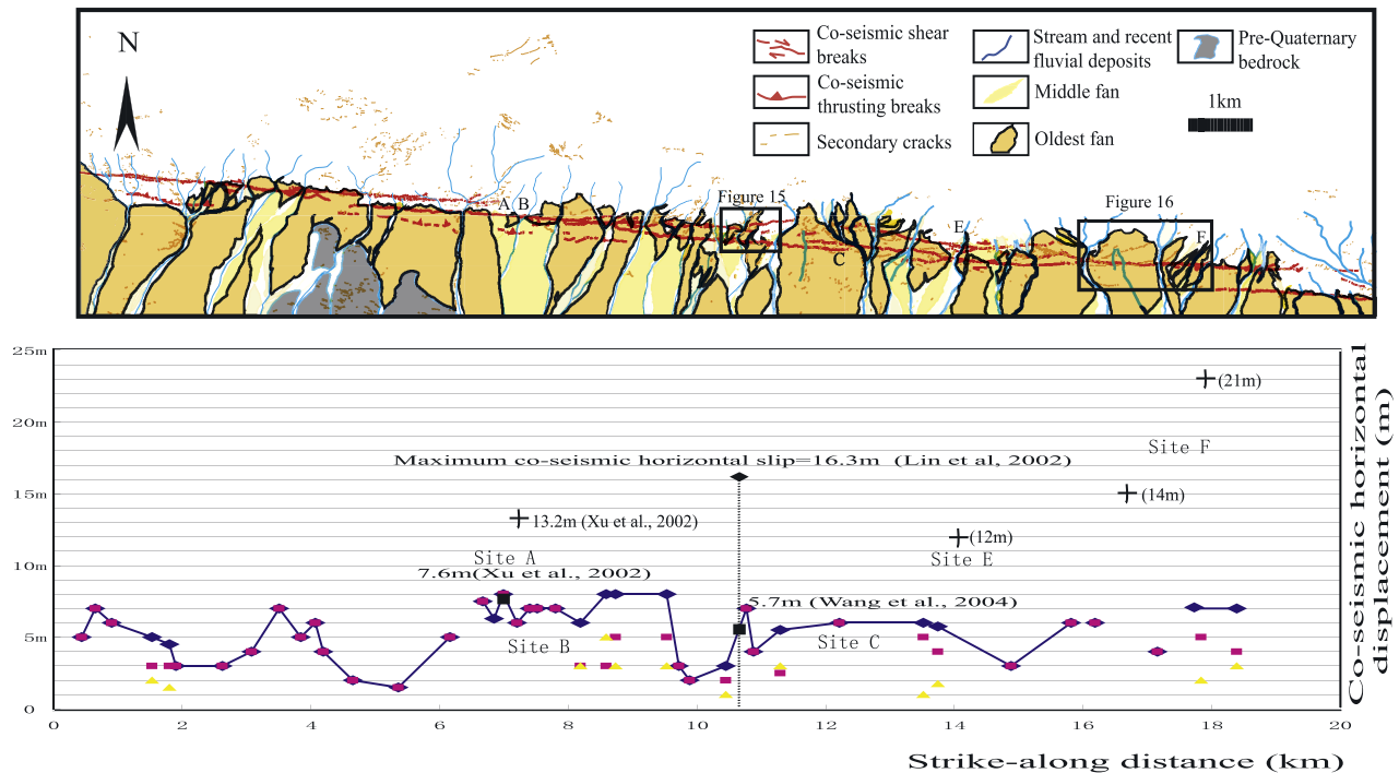
Figure 11. (a) Detailed strip map of the Yuxi Feng subsection of the Kunlunshan earthquake surface rupture zone northeast of Kusaihu Lake from 93.2500^{\circ}\text{E} to 93.4667^{\circ}\text{E} derived from Ikonos satellite images, showing a complicated structure of multiple subparallel strike-slip faulting strands with a reverse faulting strand on the south to form as wide as 550 m surface rupture zone produced directly by faulting (blank areas north of the surface rupture zone are pre-Quaternary bedrocks of Kunlun Range and black square is the location for Figures 15 and 16). (b) Coseismic left-lateral displacements identified from linear geomorphic markers on the Ikonos images and also field measurements. Yellow triangle or mauve square represents coseismic displacement on the single strand and blue rhombus the sum of the coseismic displacements on the different strands at the same site. Black cross represents the cumulative offset value.
