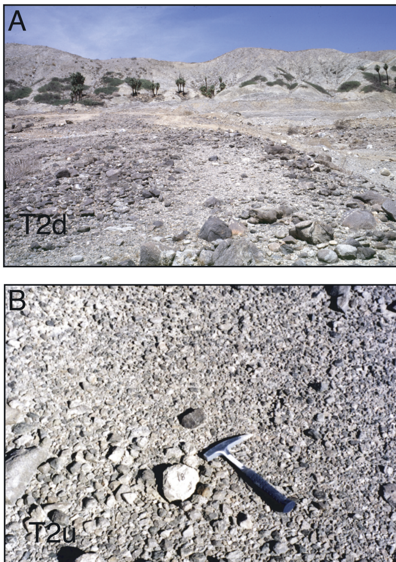
Figure 6. (a) The surface of terrace T2d, downstream of the fault zone. View to northeast, toward principal fault zone marked by aligned palm trees and by scarp. Lightly varnished cobbles paving the alluvial surface are typical of those sampled for surface exposure dating. (b) Close-up of desert pavement on T2u surface northeast of fault. The white cobble near the head of the rock hammer is sample 18 ( ^{10}\text{Be} age of 35.4 \pm 3.9 ka).
