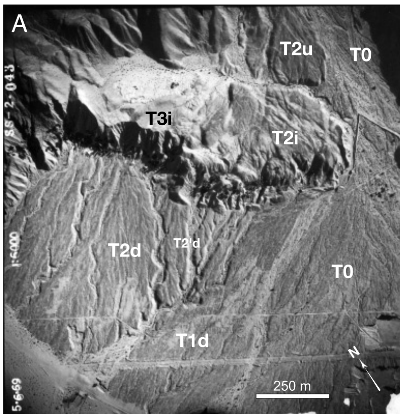
Figure 4. Vertical aerial photo of Biskra Palms site (6 May 1969). Main fan surface T2d, south of the fault, has been disconnected from its upstream counterparts T2i and T2u by right-lateral motion along the fault. Youngest alluvial surfaces are T0. T1d is an intermediate terrace.
