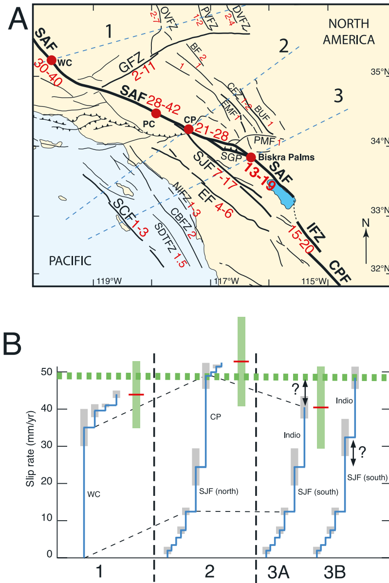
Figure 9. (a) Map of Southern California active faults. Values for slip rates on various faults and sites along SAF are from the literature (Table 2). Rates are expressed for right-lateral slip in mm/yr, except for GFZ and PMF, which are left-lateral faults. New rate at Biskra Palms is from this study. Dotted lines 1, 2, and 3 are paths along which we summed slip rates across plate boundary. WC, Wallace Creek; PC, Palett Creek; CP, Cajon Pass; OVFZ, Owens Valley Fault Zone; PVFZ, Panamint Valley Fault Zone; DVFZ, Death Valley Fault Zone; BF, Blackwater Fault; BUF, Bullion Fault; CFZ, Calico Fault Zone; EMF, Emerson Fault; PMF, Pinto Mountain Fault; SGP, San Geronio Pass; IFZ, Imperial Fault Zone; CPF, Cerro Prieto Fault; SJF, San Jacinto Fault; EF, Elsinore Fault; NIFZ, Newport-Inglewood Fault Zone; CBFZ, Coronado Bank Fault Zone; SDTFZ, San Diego Trough Fault Zone; SCF, San Clemente Fault. (b) Total slip of Pacific-America plate boundary for paths 1, 2, and 3 shown in Figure 9a. Considering an average plate boundary rate of 48–50 mm/yr (thick gray dotted line), the rate found in this study implies that either slip transfer (5–10 mm/yr) occurs toward the Eastern California Shear Zone east of our site (path 3A) or that the SJF is fast (>20 mm/yr; path 3B).
