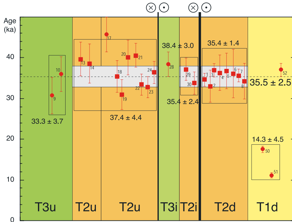
Figure 8. Plot of ^{10}\text{Be} model ages for each surface. The positions of each principal fault strand relative to the surfaces appear as vertical lines. Dotted line represents average age for T2. Light gray stripe is average standard deviation for samples represented by squares. Data are tabulated in Table 1.
