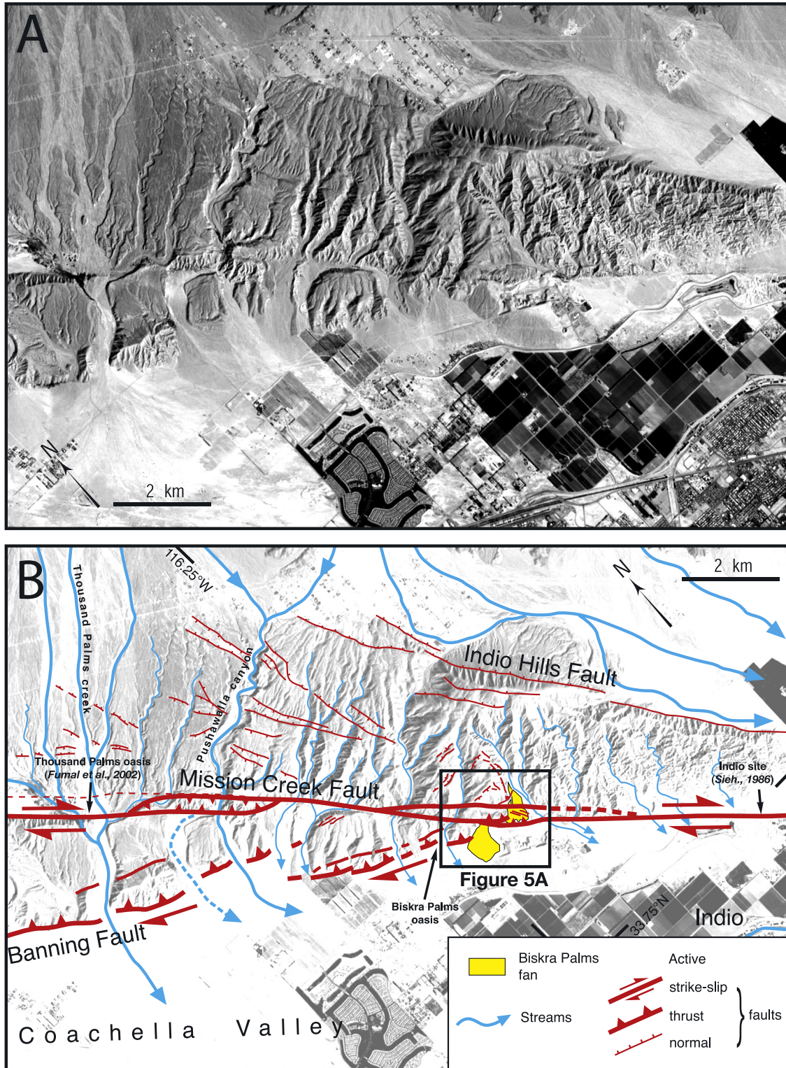
Figure 2. (a) SPOT image (KJ 545-282, 13 November 1999) of the southeastern Indio Hills. Main trace of San Andreas Fault is visible across uplifted and dissected alluvial sands and gravels of the Indio Hills. Streams that cross the main fault trace have jogs that are characteristic of right-lateral motion along the fault. (b) Interpretation of SPOT image outlining main strands of San Andreas Fault and faults across Indio Hills (modified from Clark [1984]).
