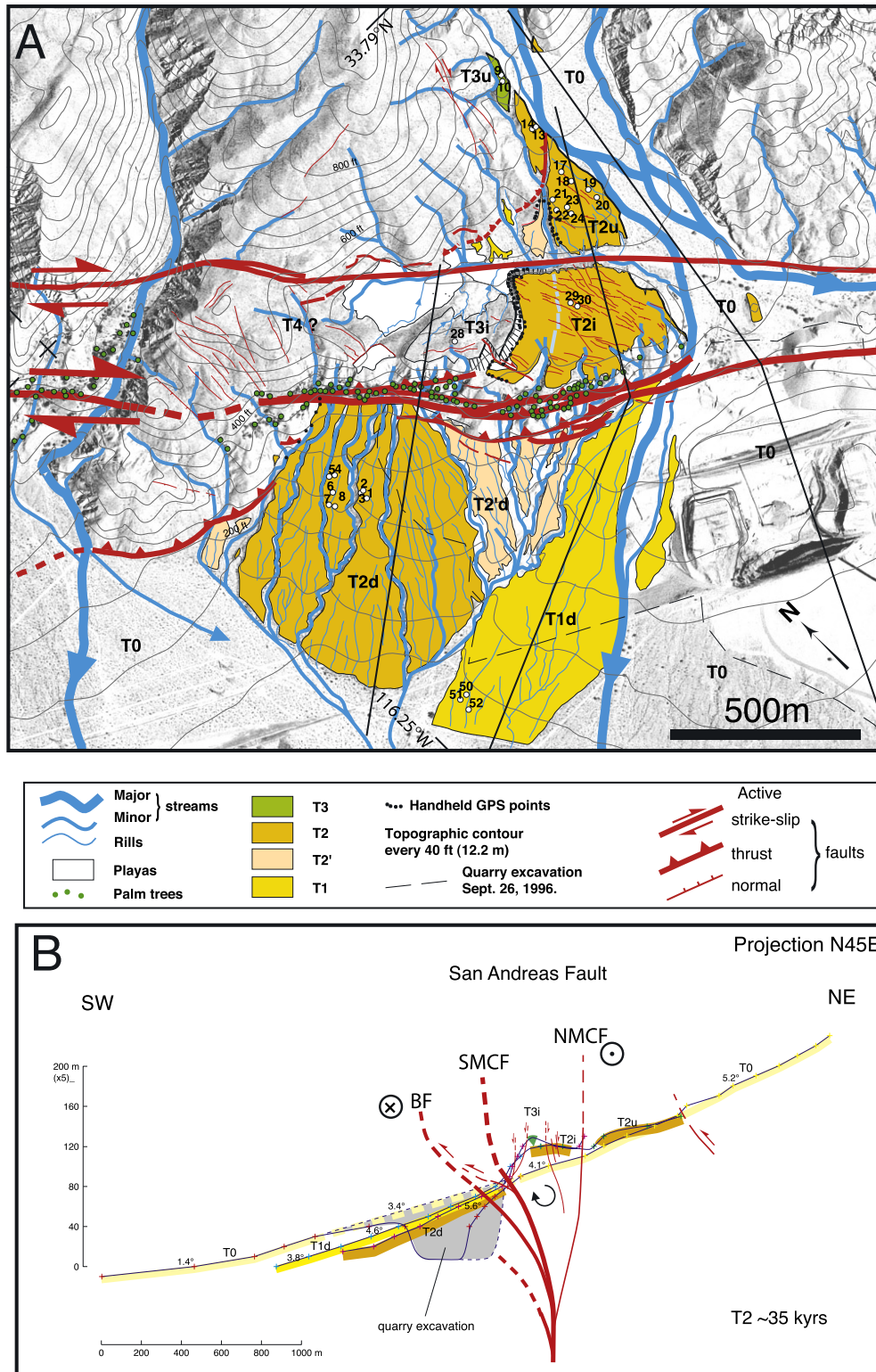
Figure 5. (a) Map of fault traces and alluvial surfaces superimposed on topographic contours and USGS orthophoto (26 September 1996). Numbered dots show locations of samples collected for cosmogenic dating. Straight lines indicate positions of topographic profiles plotted in Figure 5b. (b) Superimposed topographic profiles across main alluvial levels, projected to a line perpendicular to strike of the fault zone. Match between surfaces northeast and southwest of central fault zone is clear. Main scarp along the principal strike-slip fault is likely due to thrust component and uplift of block between the two strike-slip faults. Fault geometry at depth, though hypothetical, is consistent with this interpretation.
