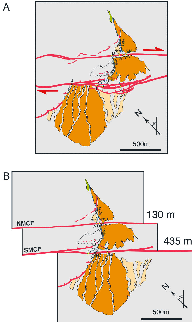
Figure 7. (a) Map of alluvial unit T2, faults and various considered piercing points. Small white dots are points surveyed in the field along piercing lines. Dashed lines are western edges of T2 that we consider for offset estimation. Lettered circles are piercing points defined by intersection of dotted lines with fault traces. (b) Preferred reconstruction of T2 surface and corresponding total offset values.
