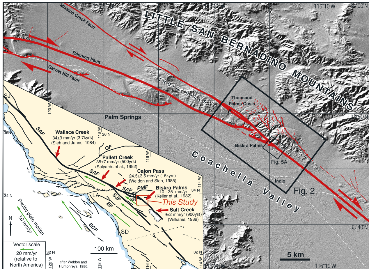
Figure 1. Map of San Andreas Fault system in the Coachella Valley. Fault map in eastern Indio Hills is modified from Clark [1984]. Biskra Palms site is located along southwestern Indio Hills, just southeast of the Biskra Palms oasis. Background is shaded DEM derived from Shuttle Radar Topography Mission data (30 m pixel). Inset, modified from Weldon and Humphreys [1986], shows Biskra Palms site in relation to other sites where geological long-term slip rate have been already determined. Gray arrows [Weldon and Humphreys, 1986] indicate relative motion of various crustal blocks relative to North American plate (SCF, San Clemente Fault; EF, Elsinore Fault; SJF, San Jacinto Fault; SAF, San Andreas Fault; GF, Garlock Fault; PMF, Pinto Mountain Fault; SG, San Gorgonio Pass fault zone; SJ, San Jose; LA, Los Angeles; SD, San Diego).
