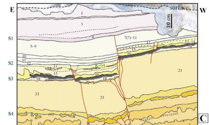
Figure 2. Photograph (A) and log (B) of wall of shallow Kazzâb-2002 trench, and log (C) of Kazzâb-2001 wall trench. K23, K24, and K29 were sampled on part of Kazzâb-2001 wall outside area shown here.
