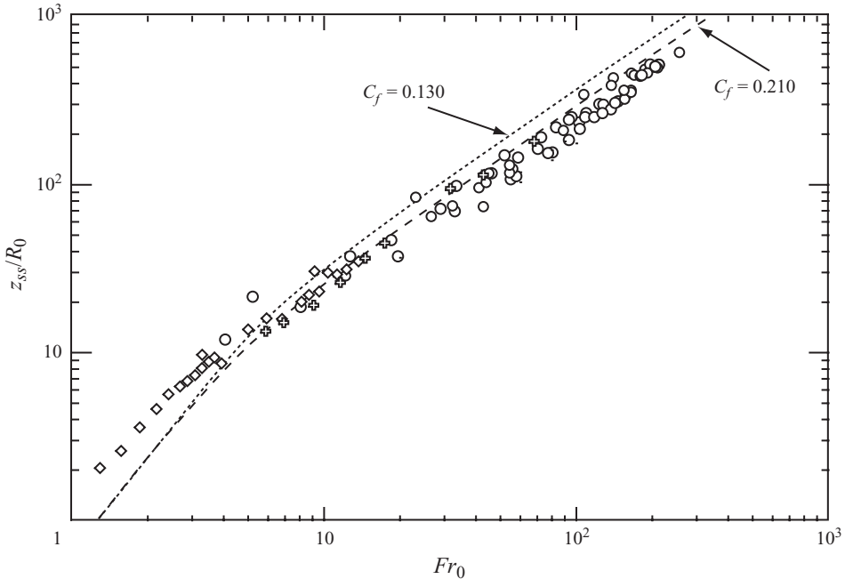
FIGURE 8. Comparison of experimental dimensionless steady-state heights with the theoretical prediction using our new model with C_f = 0.210 , A_f = 0.244 and k = 8.4 (dashed line), C_f = 0.130 , A_f = 0.244 and k = 8.4 (dotted line) for a ‘top-hat’ flow at the source. The symbols are the same as in figure 2.
