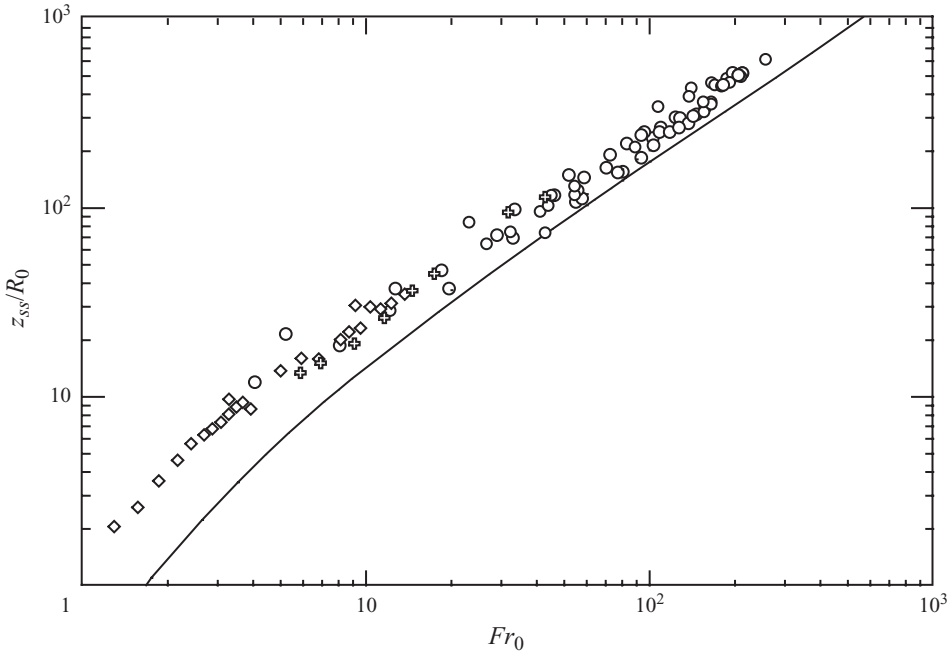
FIGURE 2. Dimensionless steady-state height ( z_{ss}/R_0 ) of experimental fountains as a function of the source Froude number compared with theoretical predictions (solid line) using the model of Morton et al. (1956) with \alpha_e = 0.1 and using z_m/z_{ss} = 1.43 as in Kaye & Hunt (2006). \circ , Baines et al. (1990); \diamond , Kaye & Hunt (2006); \clubsuit , the present study (see the Appendix). Error bars are smaller than the symbol size.
