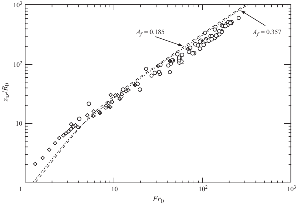
FIGURE 9. Comparison of experimental dimensionless steady-state heights with the theoretical prediction using our new model with C_f = 0.170 , A_f = 0.185 and k = 8.4 (dashed line), C_f = 0.170 , A_f = 0.357 and k = 8.4 (dotted line) for a ‘top-hat’ flow at the source. The symbols are the same as in figure 2.
