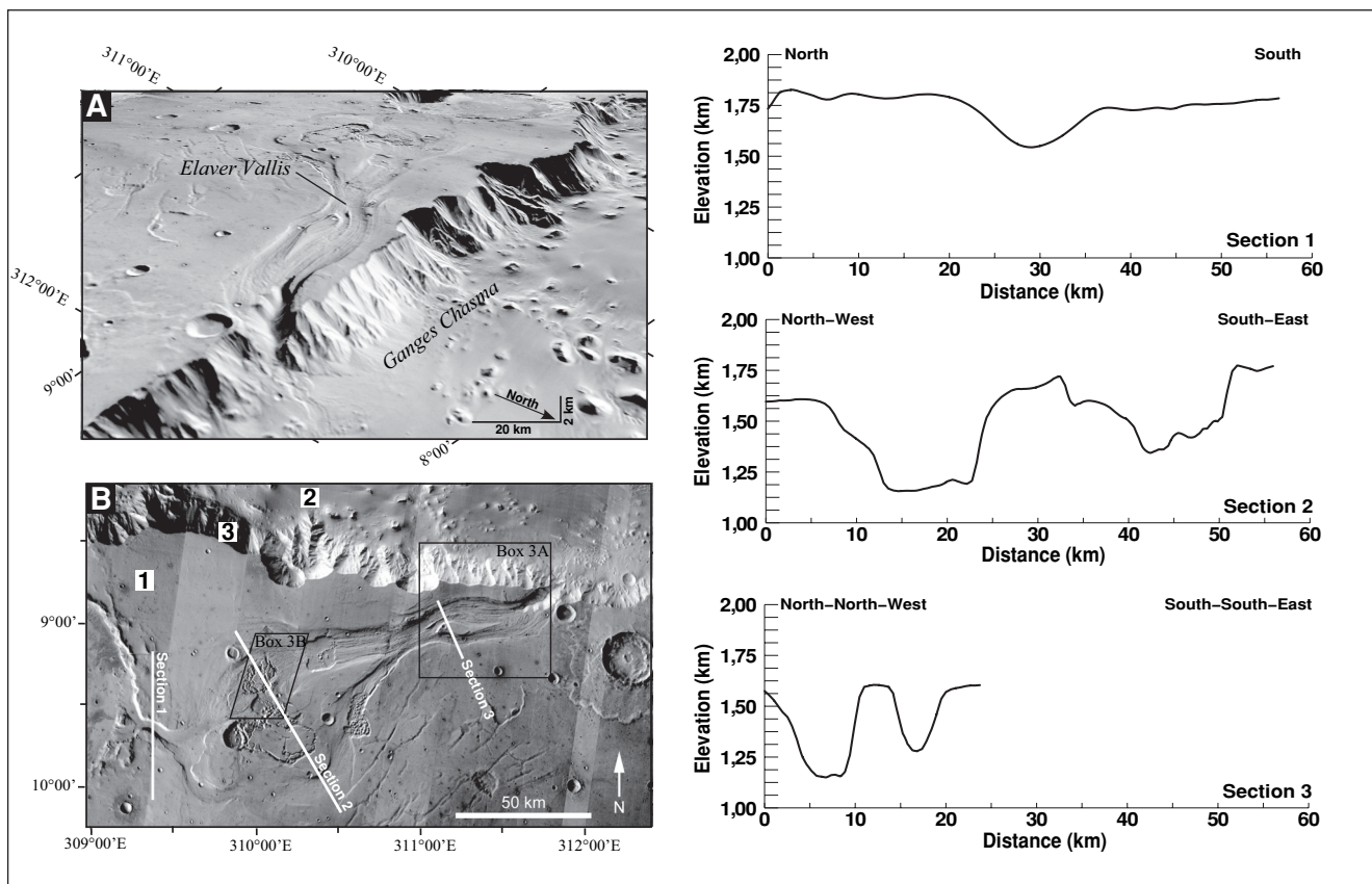
Fig. 2 – Elaver Vallis outflow channel. A: Bird's view of a day-time IR-THEMIS mosaic draped on MOLA DEM showing Elaver Vallis and its connexion with Ganges Chasma; B: Aurorae plateau noted 1, surrounds Ganges Chasma noted 2, the depression's wallslopes are noted 3. The three sections correspond respectively to topographic profiles on the right side. The down-flow slope measured between the bottom of section 1 and section 3 is smaller than 0.04 degree.
